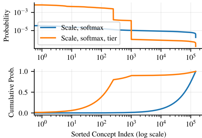
Figure 4. Learned concept sampling distribution. Given estimated scores for each of the 146,347 concepts, we need to choose how often to sample each one in order to balance exploration and exploitation. Top: we scale our scores to a desired temperature, then take the softmax to obtain a distribution over concepts. Finally, we create tiers so that the top 250 concepts have 80% of the probability mass, and the next 750 have 10%. This ensures that we sample enough from the top 1,000 concepts while still exploring other concepts with lower scores. Bottom: the top 1000 concepts are only sampled a tiny fraction of the time without tiering.
