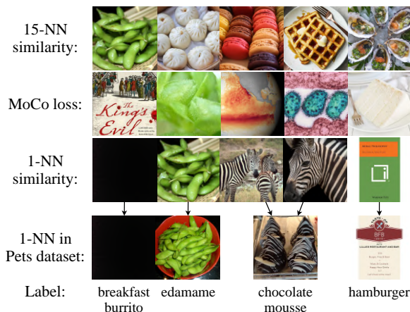
Figure 8. Most preferable images under different rewards. We show the top 5 downloaded images ranked by 3 possible image rewards on the Food dataset. 15-NN (ours) prefers a variety of food images, whereas MoCo prefers noisy images out of the training distribution. 1-NN is thrown off by outliers in the Food dataset and thus prefers black images, text, and zebras.
