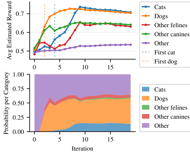
Figure 6. Self-supervised concept discovery on Pets dataset. When targeting the Pets dataset, self-supervised Internet Explorer quickly estimates high reward for concepts from the cat category (82 concepts) and dog category (246 concepts). It is also able to identify felines that are not cats (e.g., tiger) and canines that are not dogs (e.g., wolf), although it gives them lower reward on average. Finding these categories is especially challenging, since they comprise only 460/146,347 = 0.3\% of the vocabulary.
